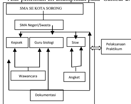
Gambar 2-1 Alur Penelitians
